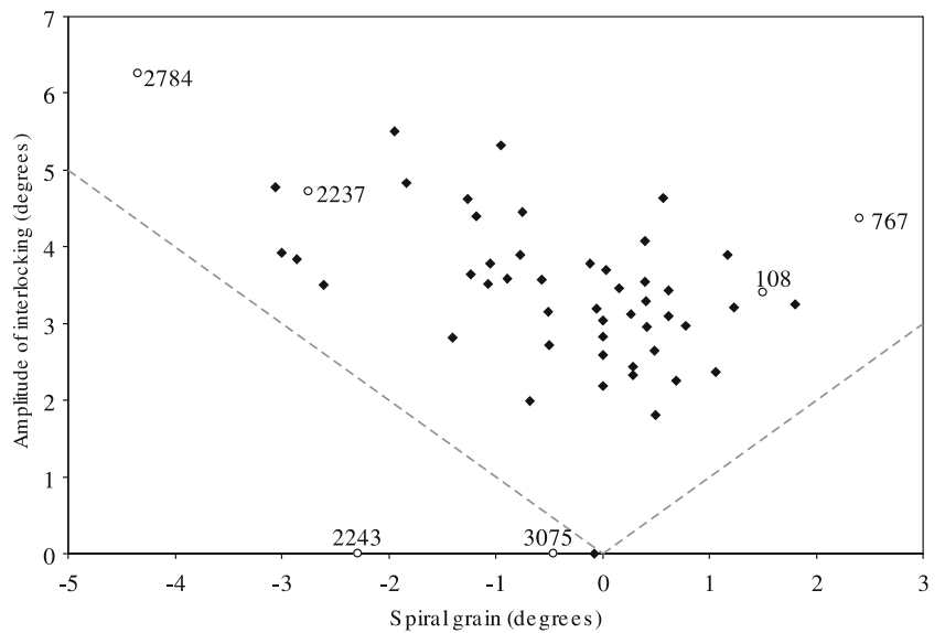
Fig. 5 Family mean estimates of spiral grain and amplitude of interlocking (solid diamonds), with the corresponding data from the six individual tree data (open circles) illustrated in Fig. 1. The dotted lines emphasise that for most families, variation in grain angle is greater than the currently-observed value
